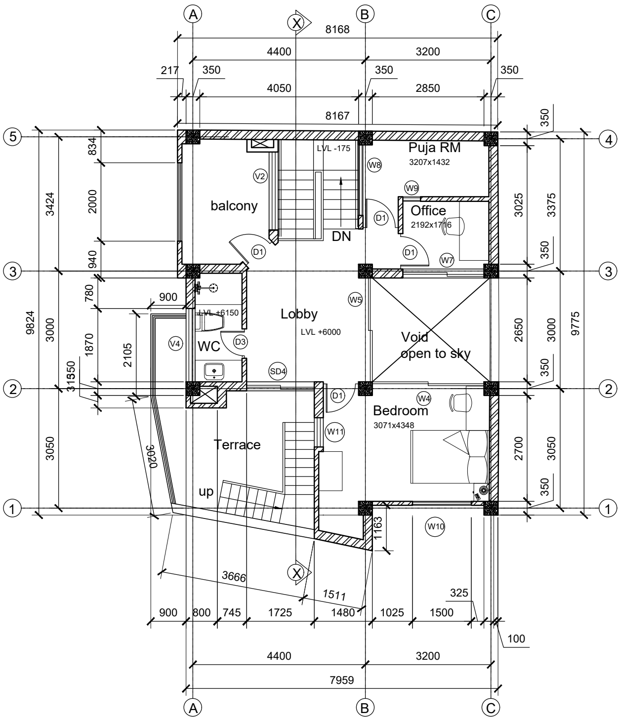
SECOND FLOOR PLAN C. Area: 61.57 sqm
